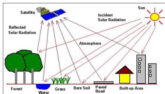
Figure 1: Illustration of the principle of remote sensing
